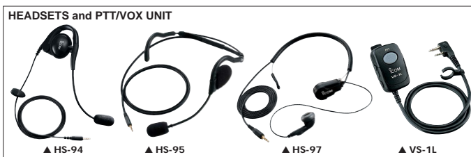
HS-94 : Earhook headset with flexible boom microphone. HS-95 : Behind-the-head headset with flexible boom microphone. HS-97 : Throat microphone fits around your neck and picks up speech vibration. VS-1L : PTT/VOX unit. Required when using these headsets with the transceiver.
