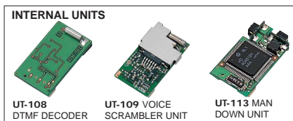
UT-108 : Provides DTMF Selective call and ANI capabilities. UT-109 (Version 02): Up to 32 scrambling codes are available. UT-110 (Version 02): Rolling type voice scrambler. Available in conventional mode only. UT-113 : Provides a man down function.
